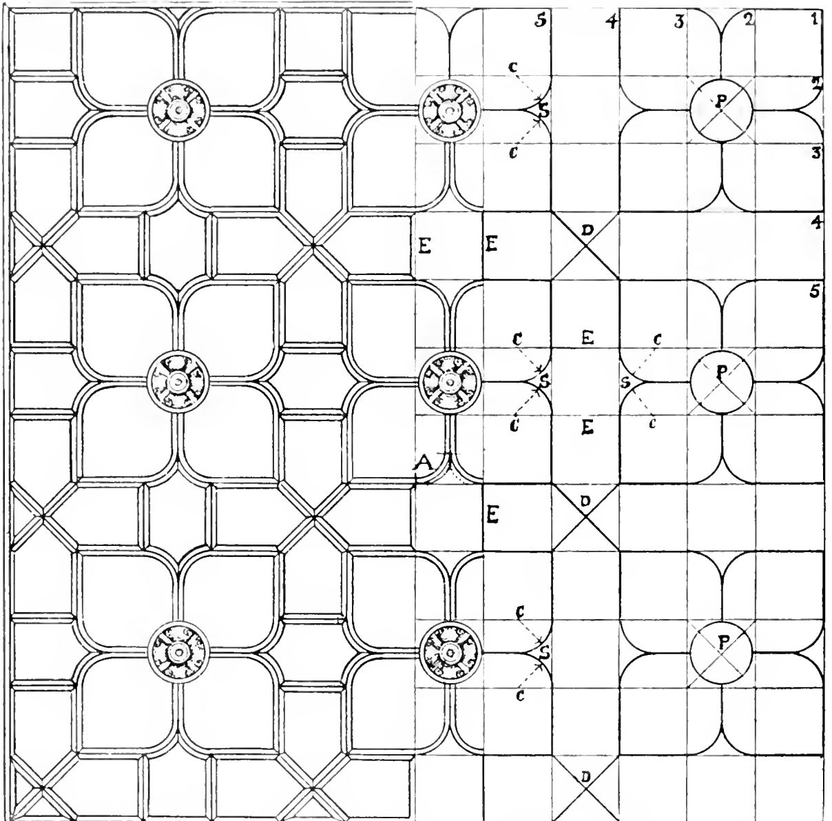
NO. 21.—PORTION OF A PLASTER CEILING, BELSACK, MIDGHTON, 1855. WITH WORKING LINES.
